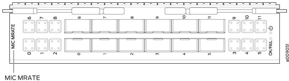
Figure 2: 12-Port Multi-Rate MIC with QSFP+
